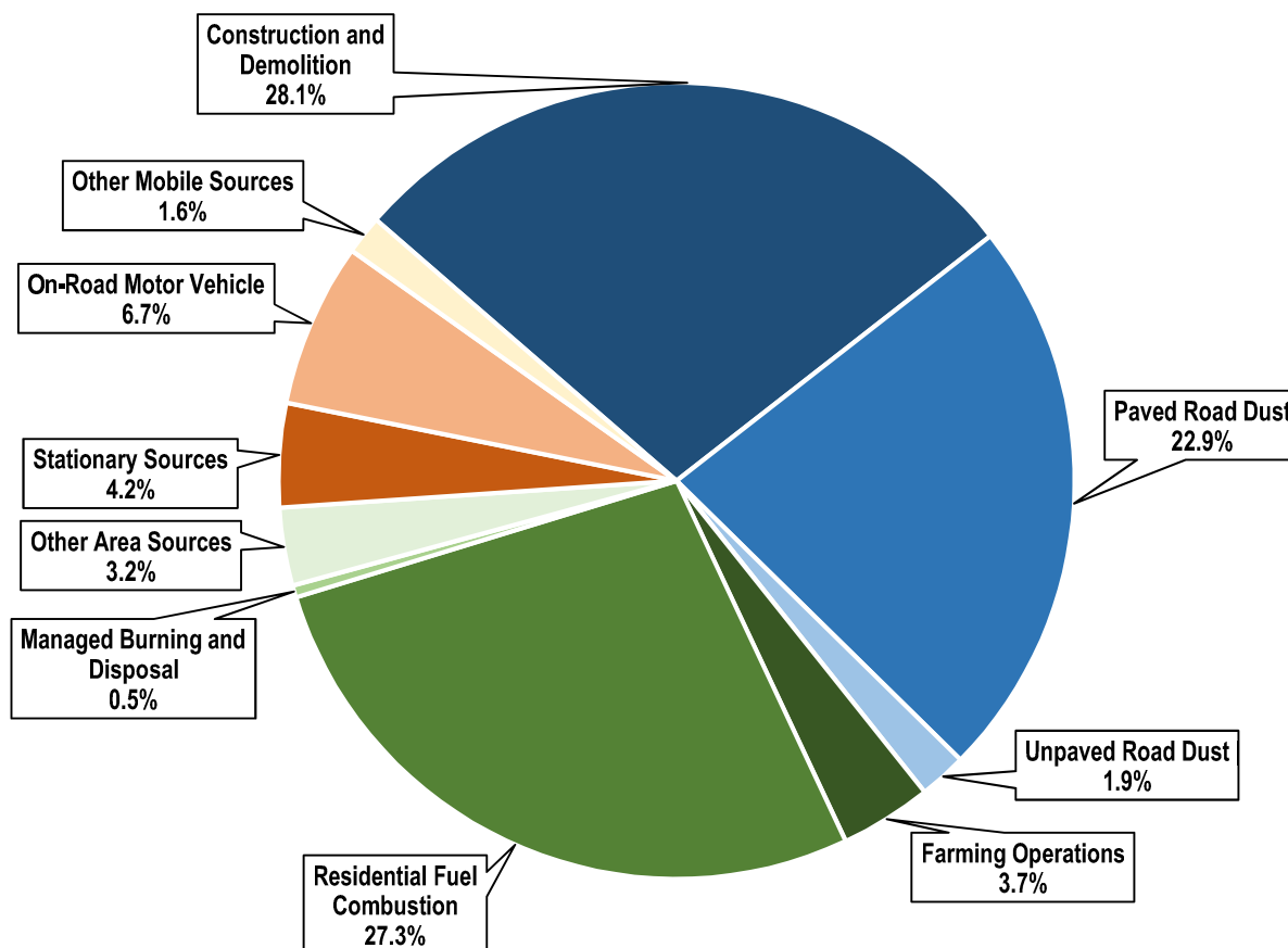
Figure 3-1 Base Year (2017) PM 10 Emissions Distribution - Sacramento County
