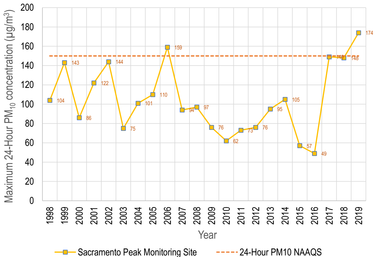
Figure 2-2 Peak 24-hour PM 10 Concentrations from 1998 – 2019 (Excluding 2018 Exceptional Events)
